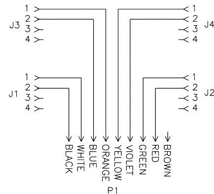
WIRING DIAGRAM
